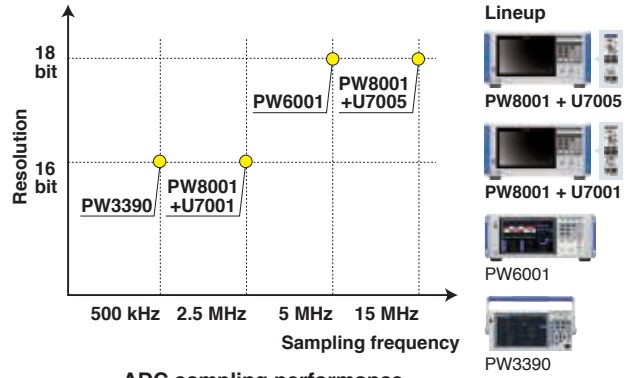
ADC sampling performance
