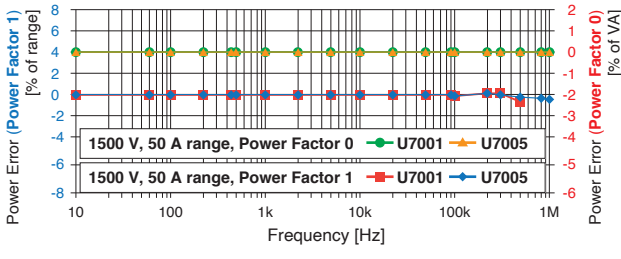
Example of active power-frequency characteristics
